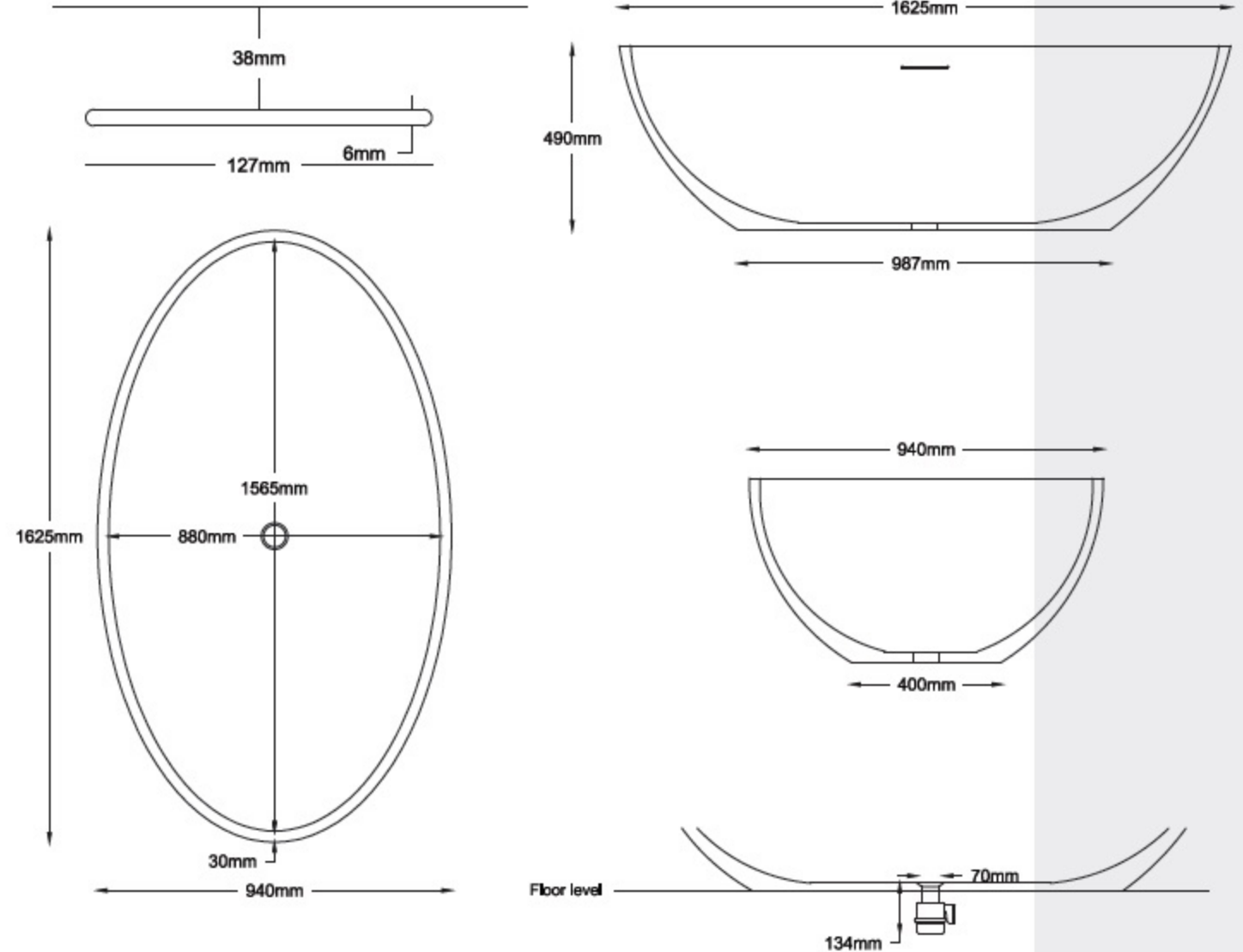
overflow detail
